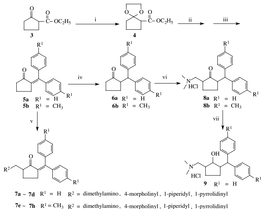
Figure 1. The synthetic pathways of compounds 5–9 .
