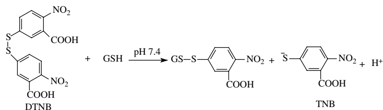
Figure 2. The interaction pathway of DTNB with GSH.
